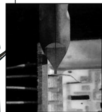
Model 50 Light Force Weld Head
